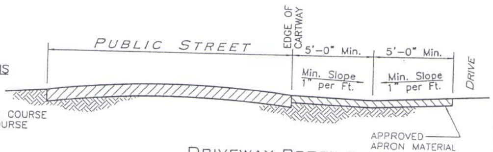
DRIVEWAY PROFILE WITHOUT DRAIN PIPE
