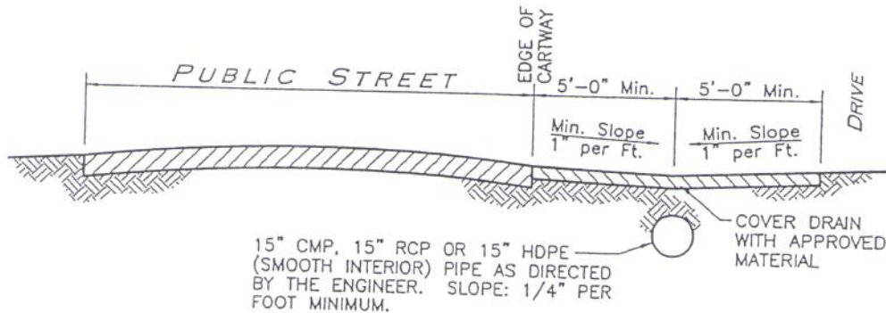
DRIVEWAY PROFILE WITH DRAIN PIPE
