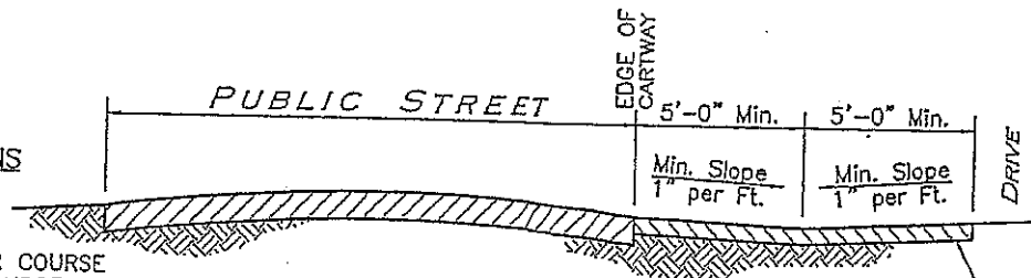
DRIVEWAY PROFILE WITHOUT DRAIN PIPE
