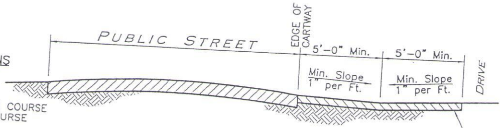
DRIVEWAY PROFILE WITHOUT DRAIN PIPE
